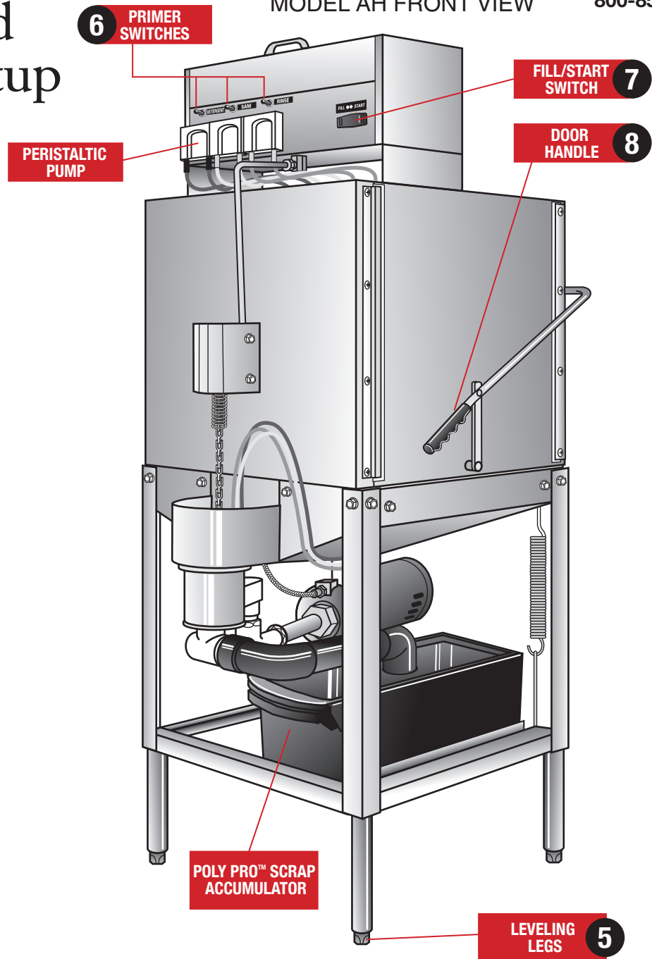
MODEL AH FRONT VIEW
