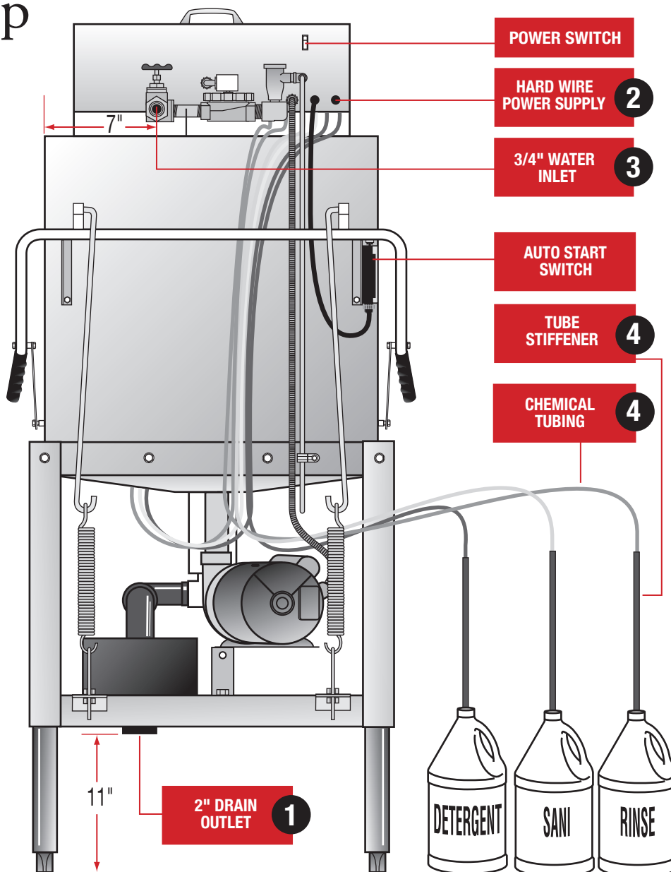
MODEL AH REAR VIEW
